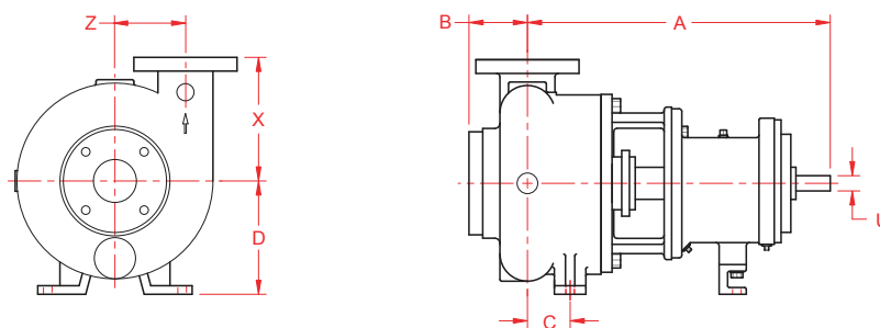
Pump Dimensions
